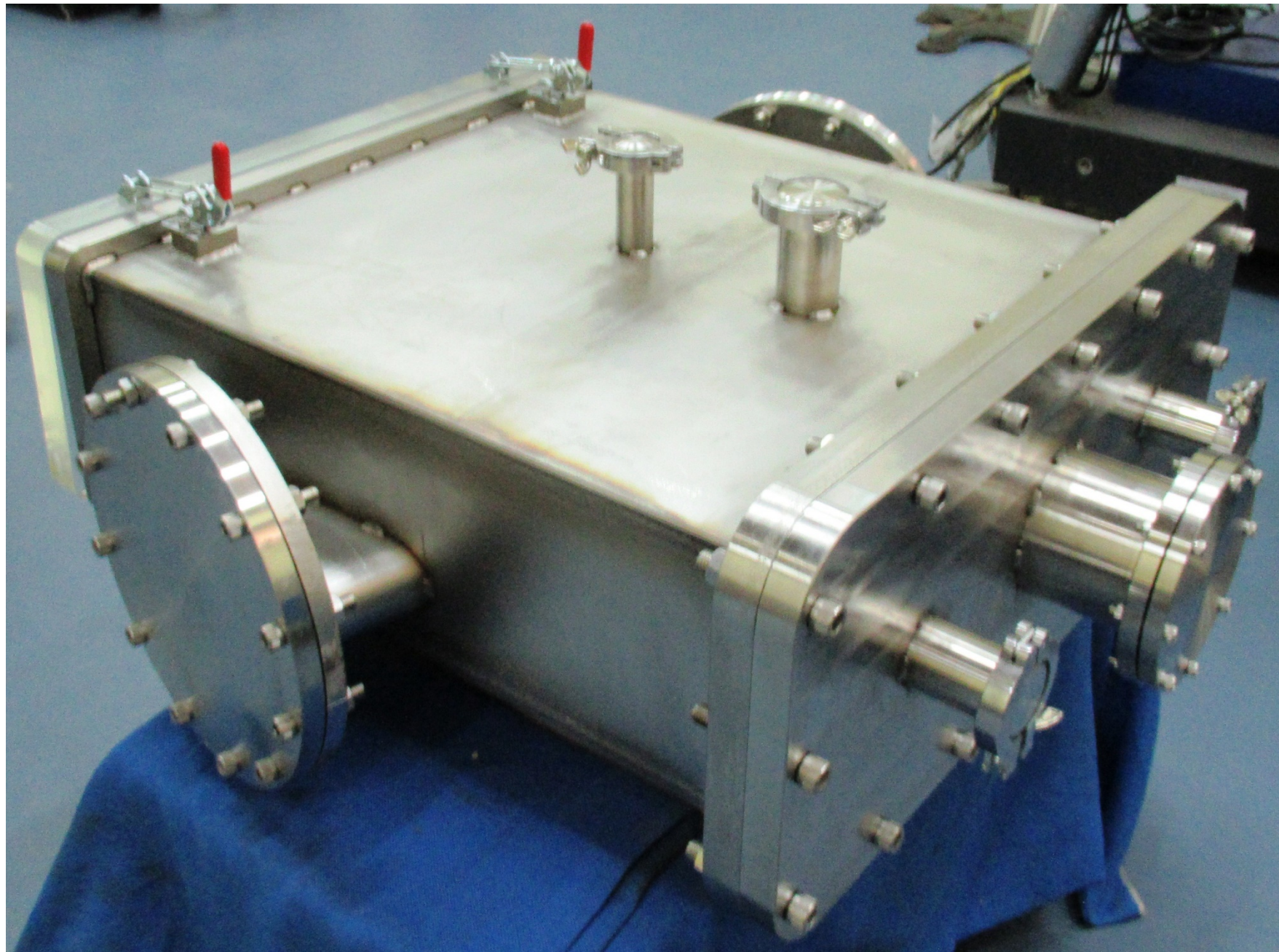
Elliptical Crystal Bender
