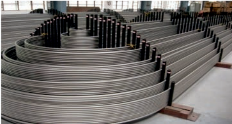
Fig.7: Incoloy-800 U bend SG tubes
