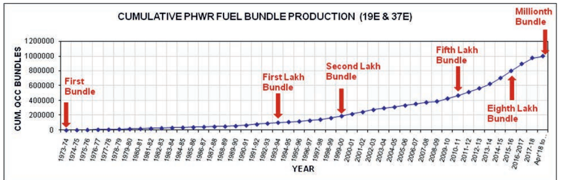
Fig. 2: Cumulative PHWR fuel bundle production over the years
