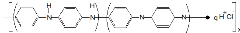
b: Empirical formula of emeraldine salt (q=1.68)
