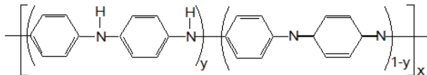
a: General Formula of Polyaniline
