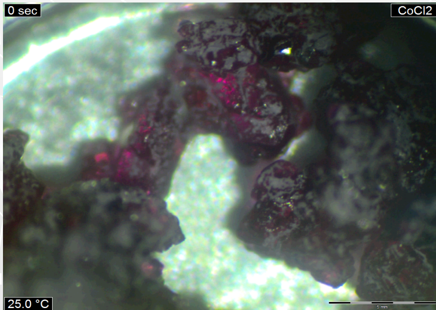
Dehydration and Thermo-chromic studies on BaCl 2 .2H 2 O and CoCl 2 .6H 2 O using DSC - Microscopy System
