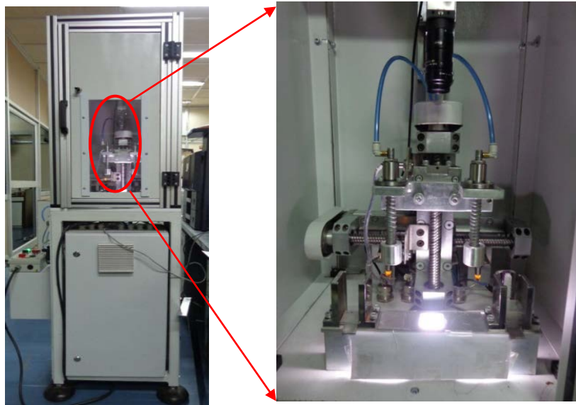
Fig. 2a (left): Automated system for batch processing; Fig.2b (right): Close-up view of the mechanism
