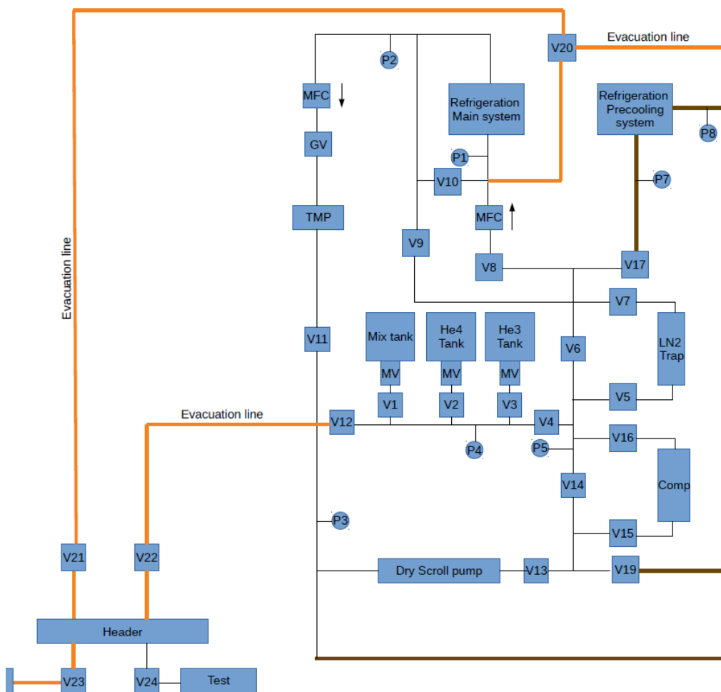
Gas flow control valve system
