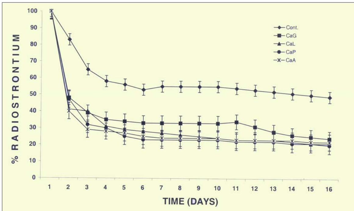
Fig. 2: Whole body retention of radiostrontium (oral)
