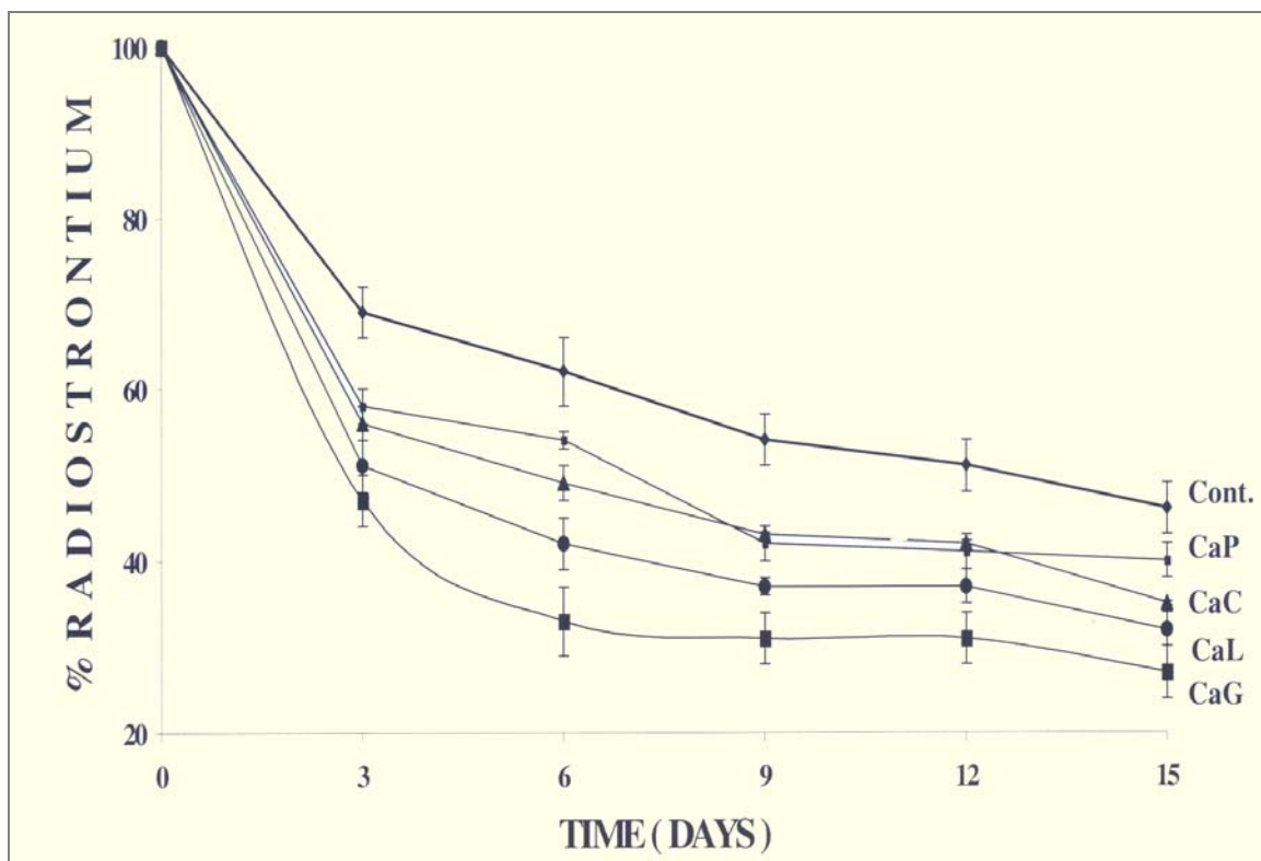
Fig. 1: Whole body retention of radiostrontium (i.p.)
