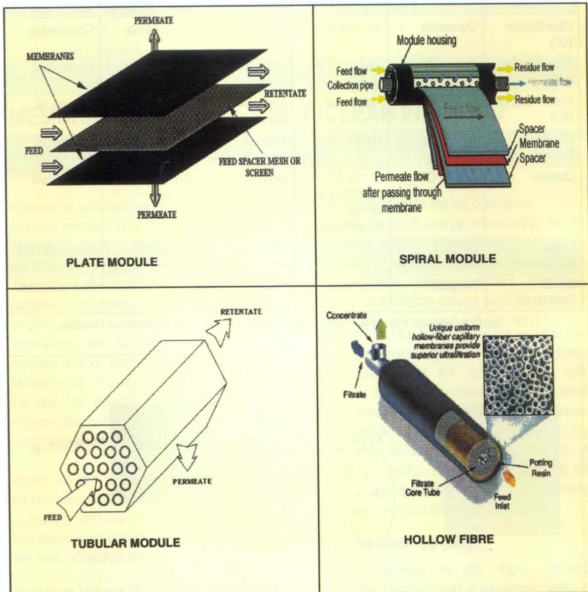
Fig. 2: Different configurations of Reverse Osmosis modules
