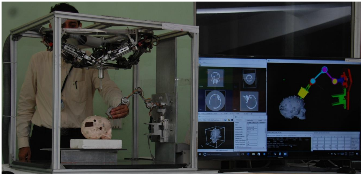
Neuro-registration procedure demonstrated using SCMM
