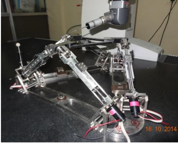
A 6 DOF Parallel Kinematic Mechanism (6D PKM) Robot for Stereotactic Neurosurgery
