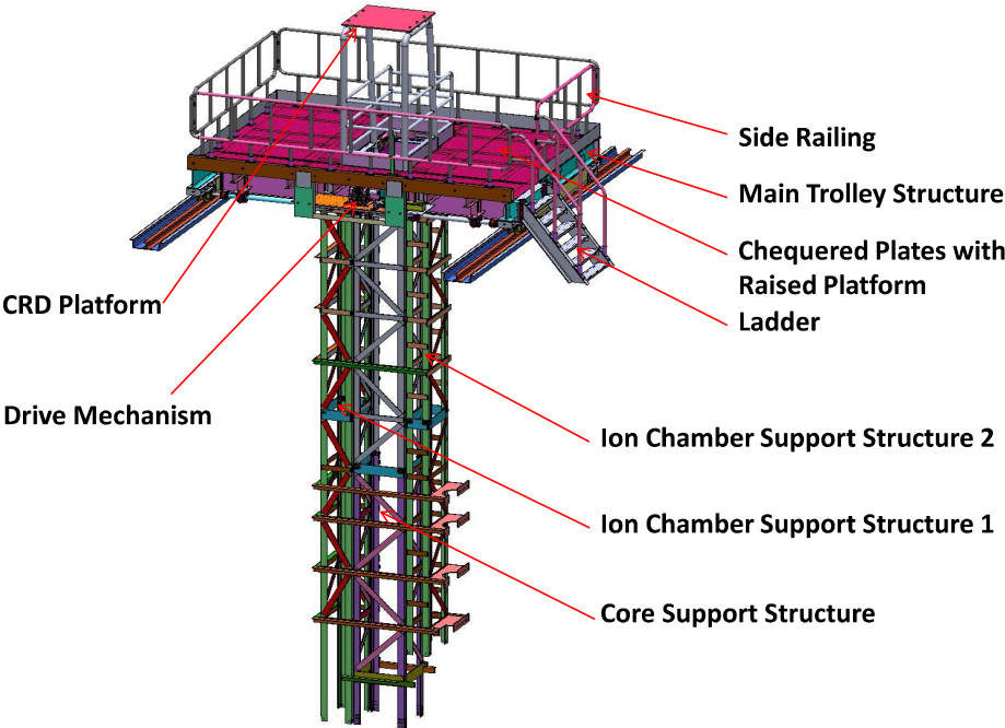
Fig: Automated Core Handling System for Upgraded Apsara Reactor
