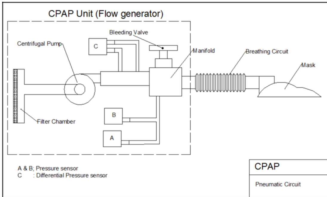
Figure 3: Pnumatic Circuit of DEAP
