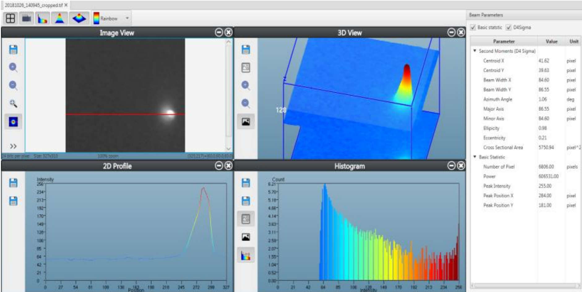
X-Ray beam profile (Image view, 3D View, 2D Profile & Histogram) of BL21 beam-line image.
