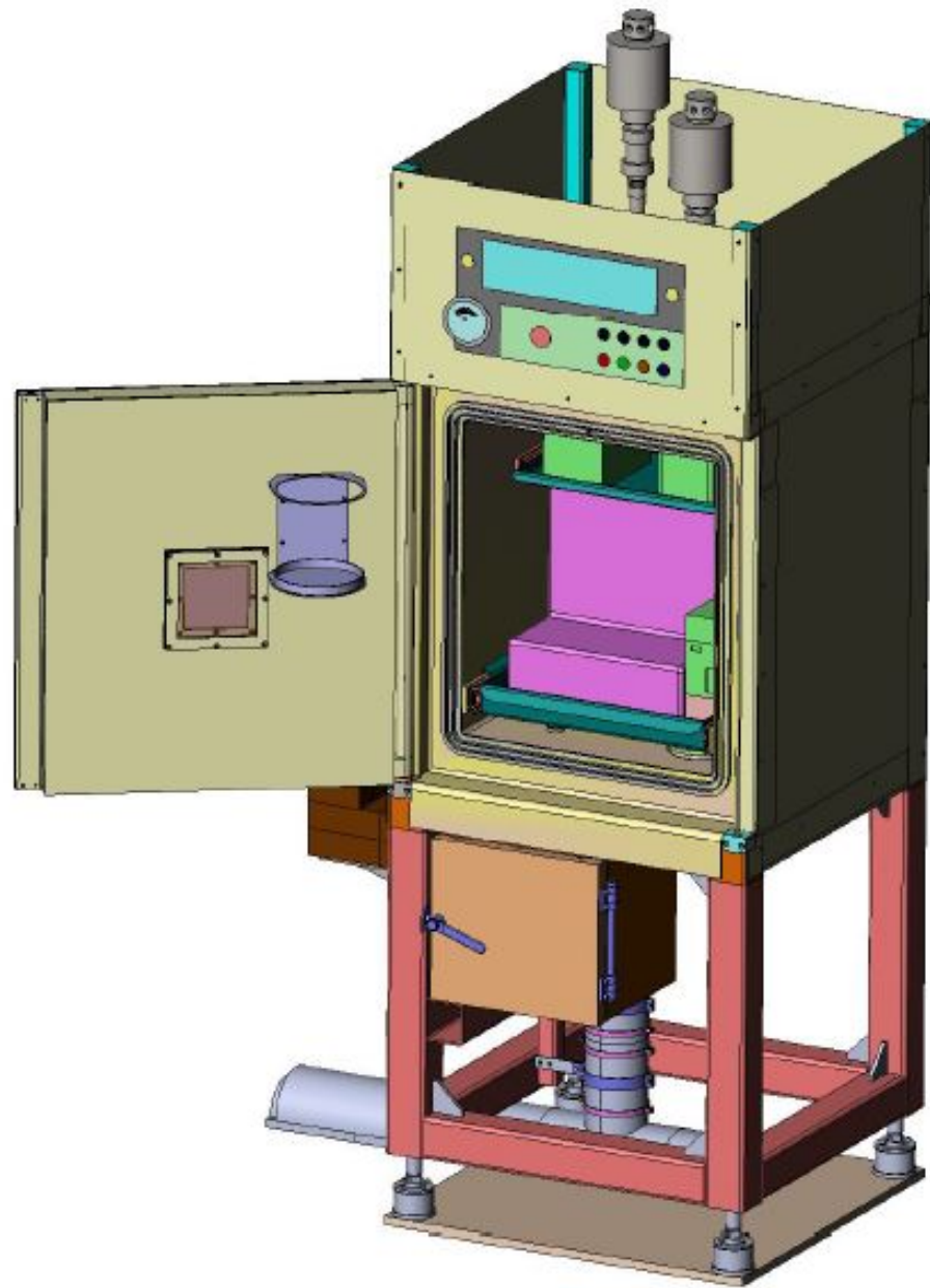
Lead Shielded Mini Hot Cell
