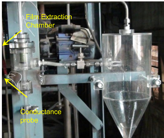
Air-Water Experimental Facility
